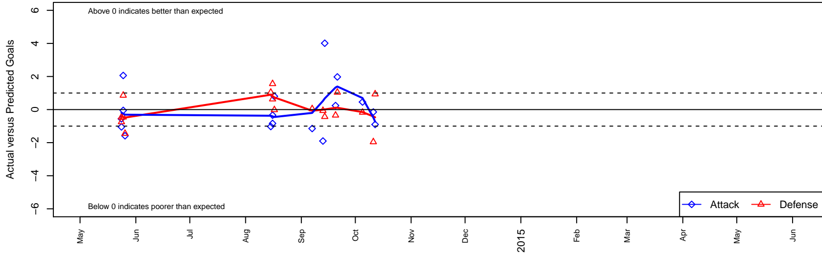
4H Chelsea G00 Dots are actual minus expected GF (blue circles) and GA (red triangles). Blue line is smoothed change in attack strength. Red is smoothed change in defense strength.
